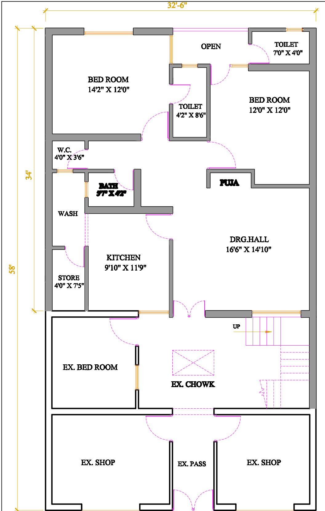
GROUND FLOOR PLAN (ALT-04)
