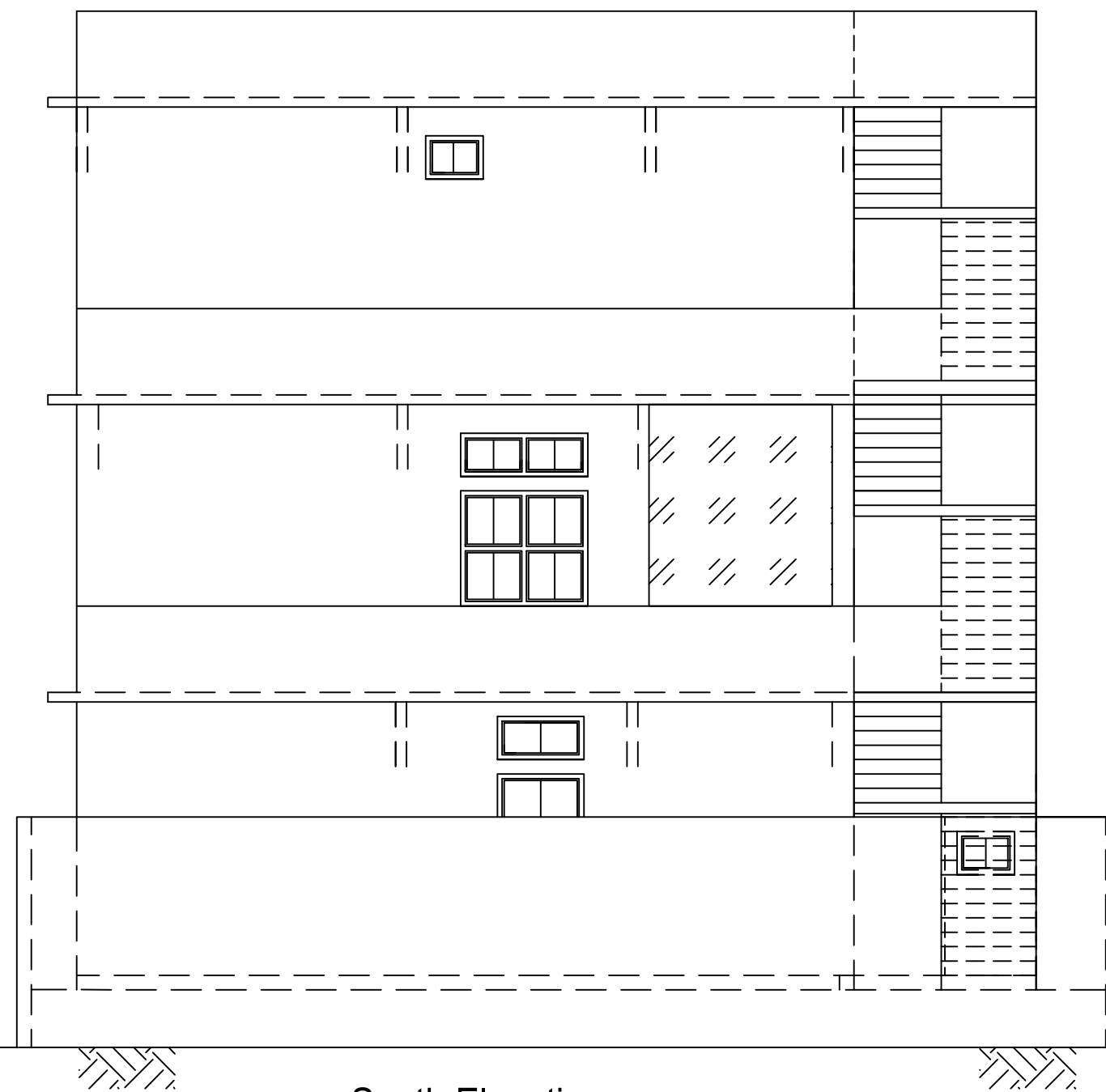
South Elevation 27/12/12
