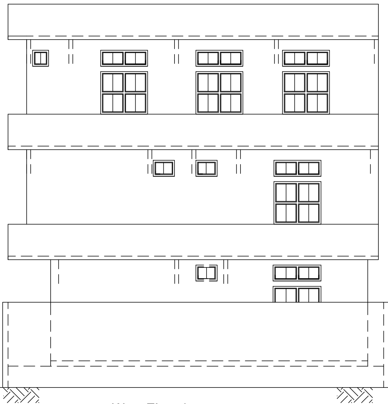
West Elevation 27/12/12
