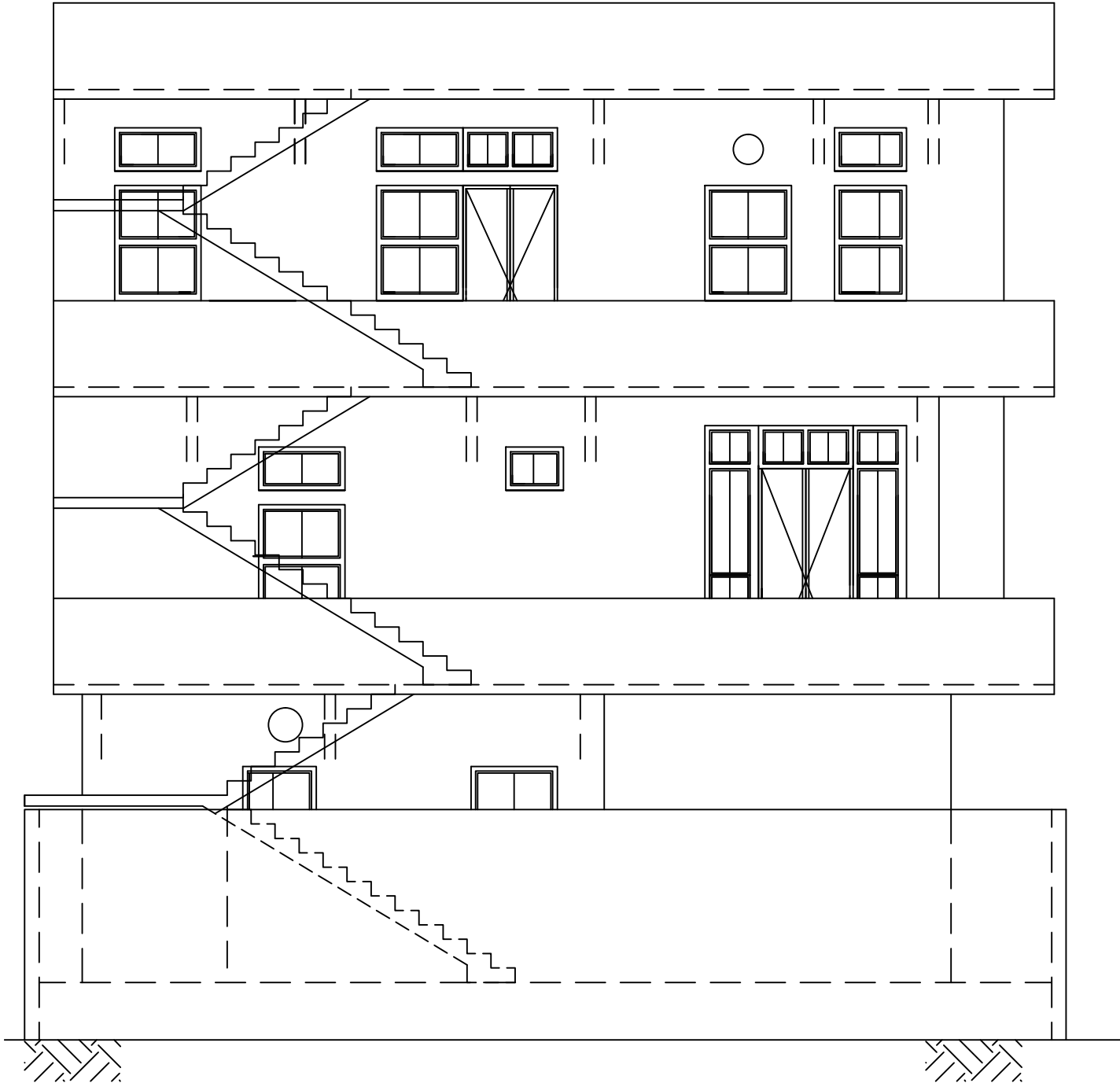
East Elevation 27/12/12
