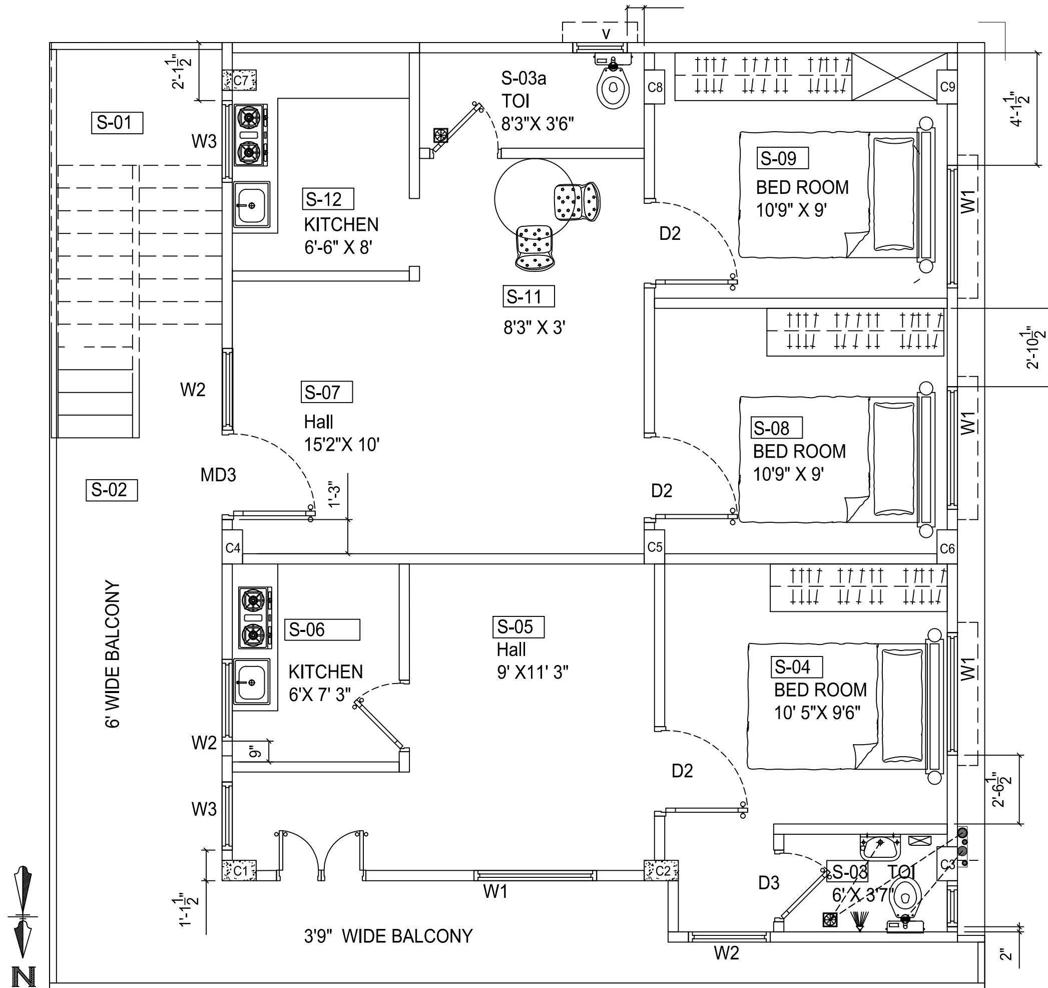
Second Floor Plan 27/12/12
